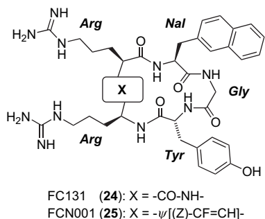
Figure 2. FC131 and its cyclic fluoroalkene pseudopeptide (FCN001). Nal= L-3-(2-naphthyl)alanine.
